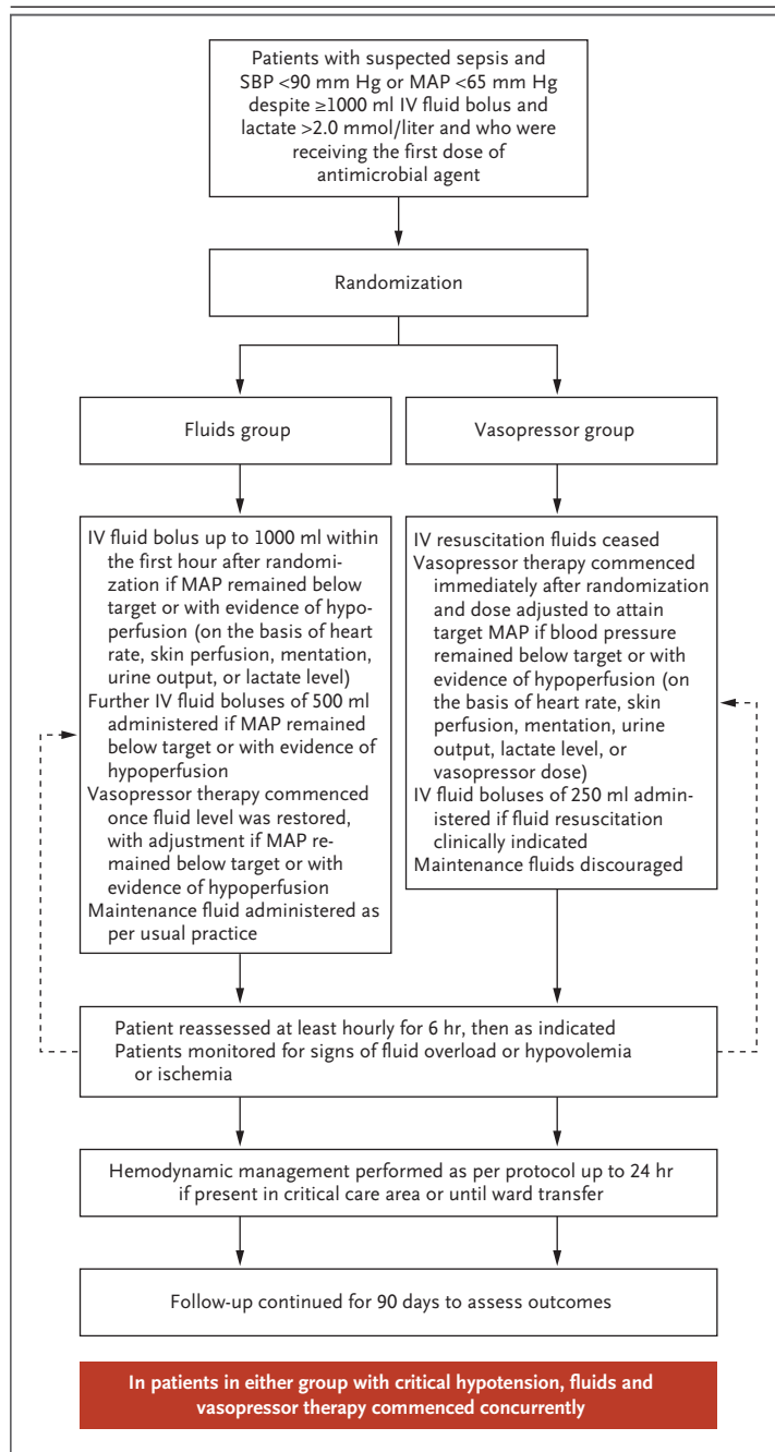
Figure 1. Trial Algorithm.
