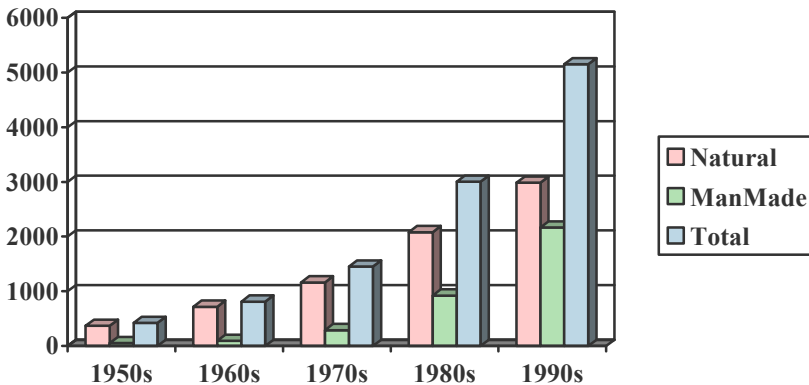
Fig. 2. Frequency of Disasters Each Decade.
